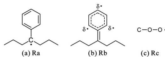
Fig. 3. The chemical structures of Ra, Rb, and Rc.
