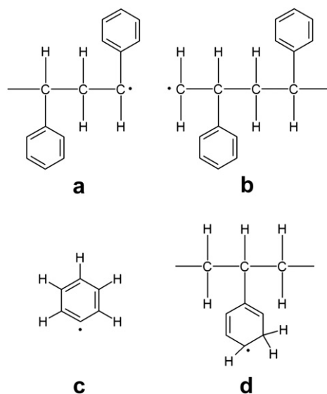
Fig. 4. Other possible radicals produced from \gamma -ray irradiation: radicals in (a) and (b) are generated from main-chain breakage, the phenyl radical (c) is produced from side-chain breakage, and the cyclohexadienyl radical (d) is generated by trapping of a hydrogen atom suggested in the literature.
