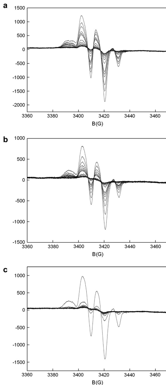
Fig. 5. Evolution of the EPR spectra of sPS irradiated with 10 kGy and annealed at (a) 65, (b) 80, and (c) 90 °C. The traces from top to bottom at \sim 3405 G in (a)–(c) represent increasing time from t = 0 min to t = 5 h.
