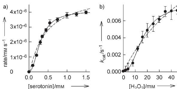
Figure 4. a) Aerobic oxidation of serotonin by 1.47 \mu\text{M CuA}\beta_{1-40} in 100.0 \text{ mM HEPES} buffer solution at \text{pH } 7.0 and 25 \text{ }^\circ\text{C} . Dashed traces are fittings to pre-equilibrium kinetics, whereas the solid traces are fittings to the Hill equation, which indicates the presence of cooperativity. b) Oxidation of serotonin by \text{CuA}\beta_{1-40} in the presence of \text{H}_2\text{O}_2 as in (a).
